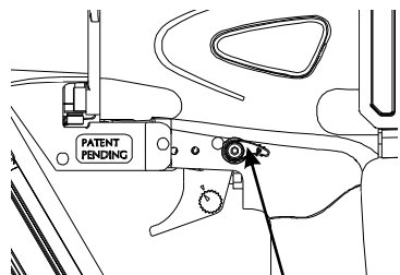
Locking mechanism(B)
